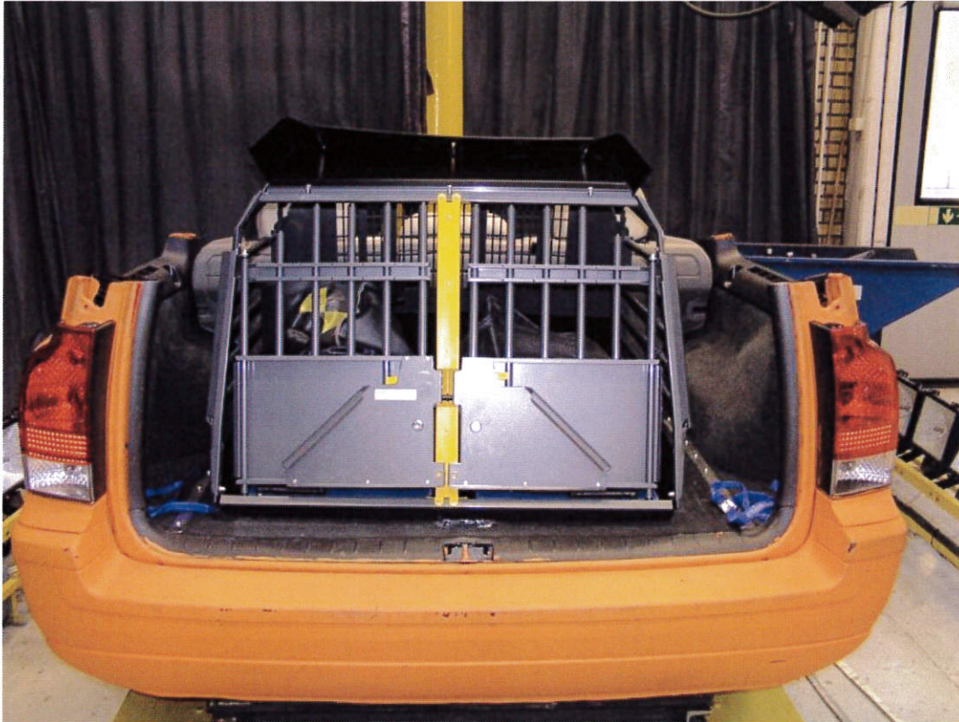
05 – After test, frontal impact
