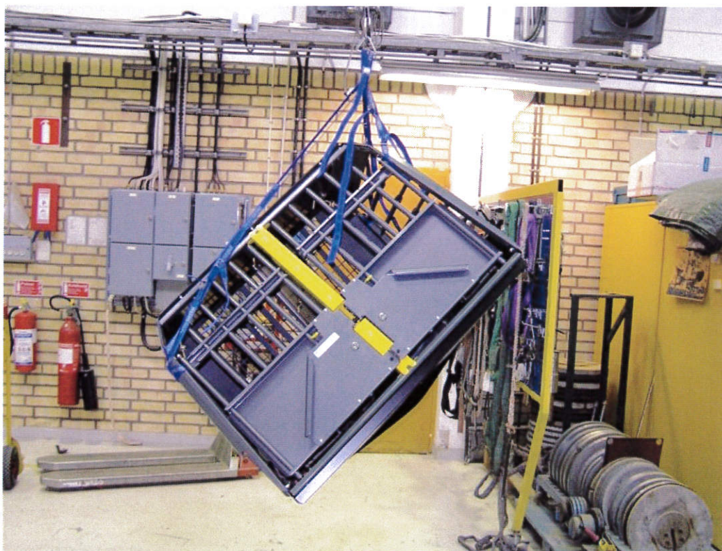
02 – Before test, Drop test
