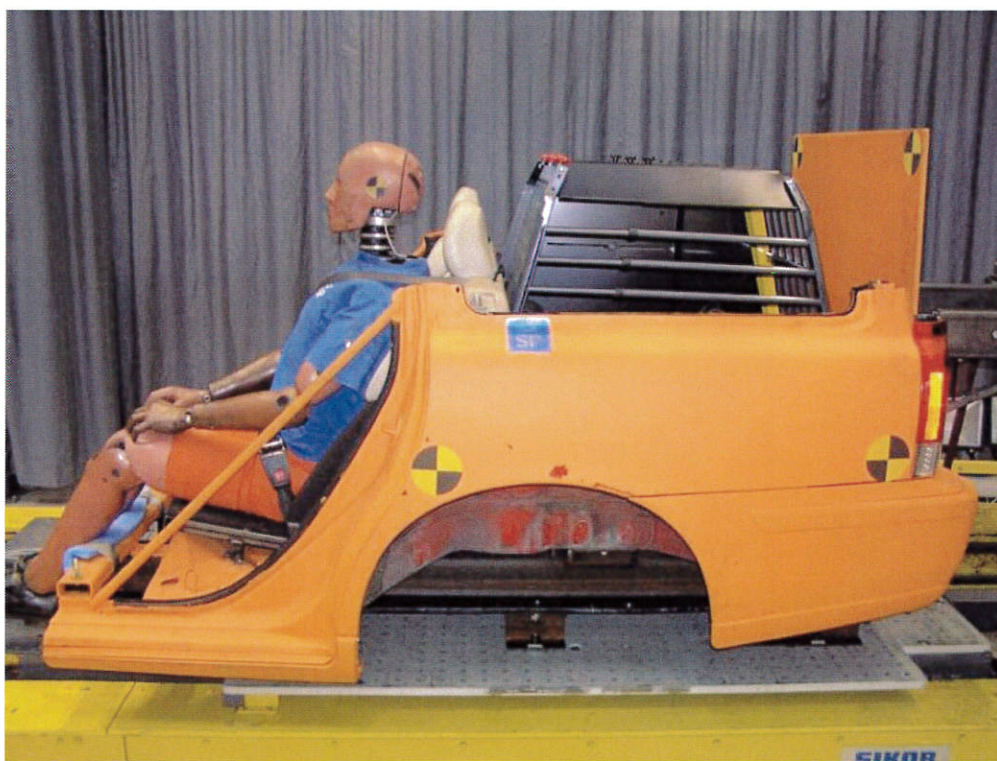
Figure 2 Test setup Rear impact test
