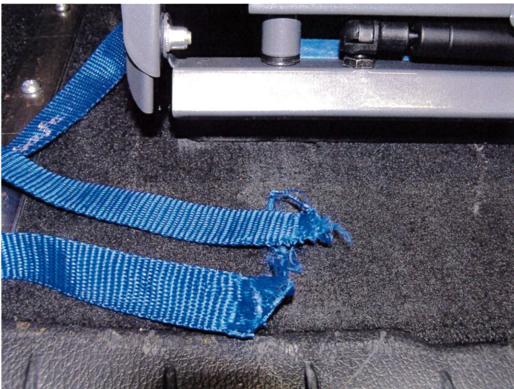
08 – After test, frontal impact
